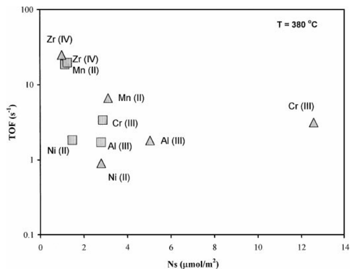
FIG. 7. Comparison of specific activity (TOFs) and surface active sites density ( N_s ) of ( \blacktriangle ) bulk metal molybdates and ( \blacksquare ) monolayer molybdenum oxide supported catalysts.
