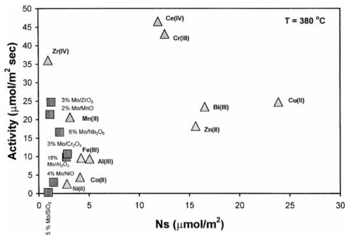
FIG. 6. Comparison of reaction rate and surface active sites density ( N_s ) of ( \blacktriangle ) bulk metal molybdates and ( \blacksquare ) monolayer molybdenum oxide supported catalysts.
